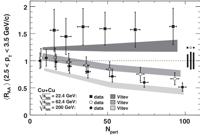
FIG. 3. The average R_{AA} in the interval 2.5 < p_T < 3.5 GeV/ c as a function of centrality for Cu + Cu collisions at \sqrt{s_{NN}} = 22.4, 62.4 , and 200 GeV. The shaded bands represent jet-quenching calculations at three discrete centralities ( N_{part} \sim 10, 50, 100 ) [22,23]. The boxes around unity represent the normalization and \langle N_{coll} \rangle uncertainties for a typical N_{coll} uncertainty of 12%.
