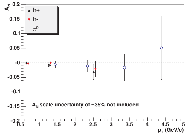
FIG. 2 (color online). Midrapidity neutral pion and charged hadron transverse single-spin asymmetry A_N vs transverse momentum. Points for positive hadrons have been shifted down by 50 MeV/c to improve readability. The error bars indicate statistical uncertainties.
