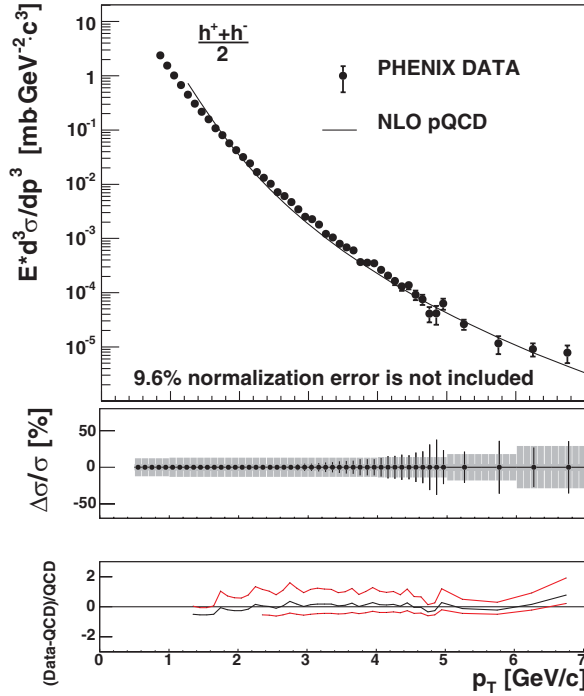
FIG. 1 (color online). Top panel: Invariant cross section vs p_T for the production of charged hadrons at midrapidity, averaged over sign. A 9.6% normalization uncertainty is not shown. The curve represents a NLO pQCD calculation at a renormalization scale of p_T [26]. Middle panel: The relative statistical (points) and point-to-point systematic (band) errors. Bottom panel: The relative difference between the data and the theory with scales of p_T/2 (lower curve), p_T , and 2p_T (upper curve).
