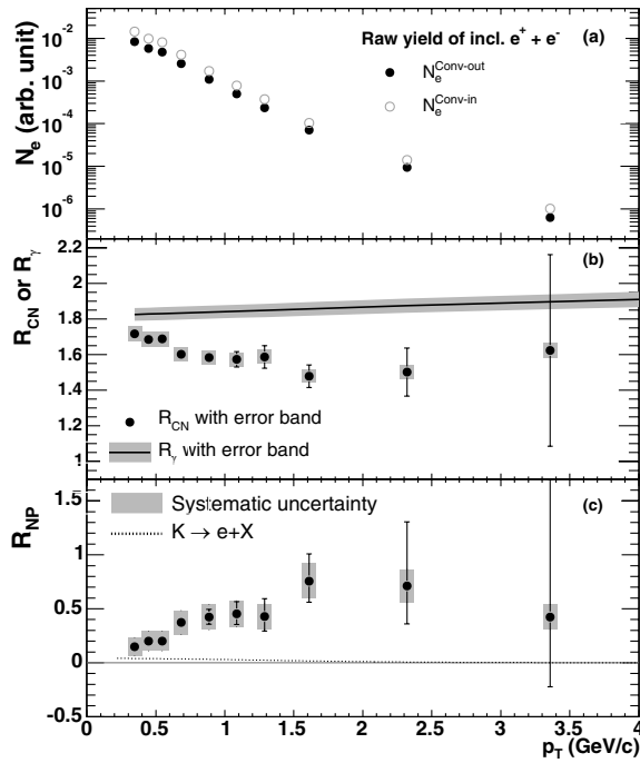
FIG. 1. Shown vs p_T (a) raw e^\pm spectra measured with the converter in (open circles) and out (closed circles). (b) Ratio of the converter in/out e^\pm yields ( R_{CN} , points) and ratio of photonic e^\pm yield with/without the converter ( R_\gamma , line and shaded band). (c) Ratio of nonphotonic to photonic e^\pm yields ( R_{NP} , points) and contribution from kaon decays (dashed line).
