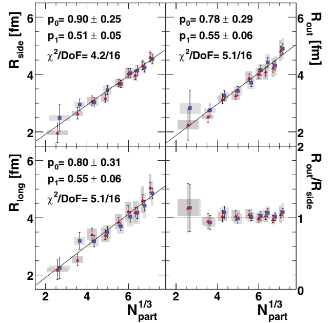
FIG. 4 (color online). Bertsch-Pratt radius parameters versus the cube root of the number of participants ( N_{\text{part}}^{1/3} ) for \pi^+ \pi^+ (blue square) and \pi^- \pi^- (red triangle) for the fits to a core-halo structure by Eq. (2) with statistical error bars and systematic error bands, in the 0.2 < k_T < 2.0 GeV/c range, with \langle k_T \rangle \sim 0.45 GeV/c. The solid line shows fits to p_0 + p_1 * N_{\text{part}}^{1/3} for both signs.
