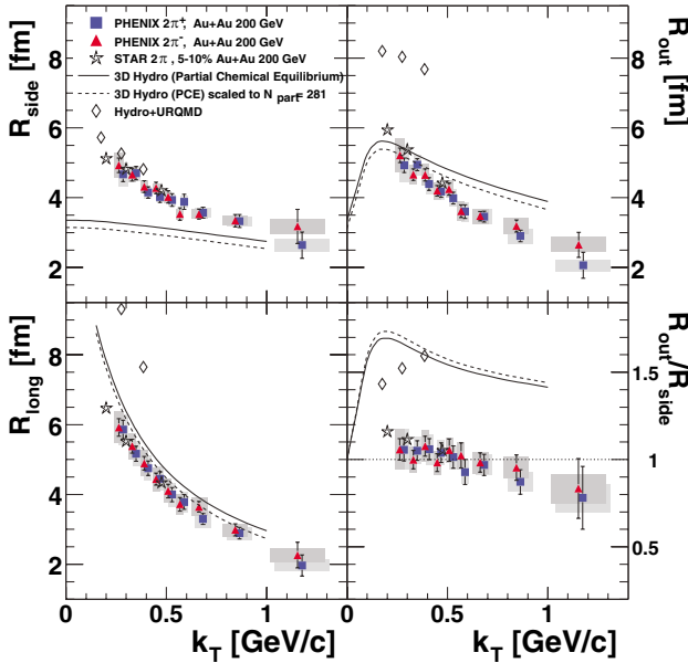
FIG. 3 (color online). The k_T dependence of the Bertsch-Pratt radius parameters for \pi^+ \pi^+ (blue square) and \pi^- \pi^- (red triangle) for 0%–30% centrality, from fits to a core-halo structure by Eq. (2), with statistical error bars and systematic error bands. Results from STAR [28] and hydrodynamics models (Hirano [29], solid and dashed lines, and Soff [30], diamonds) are overlaid.
