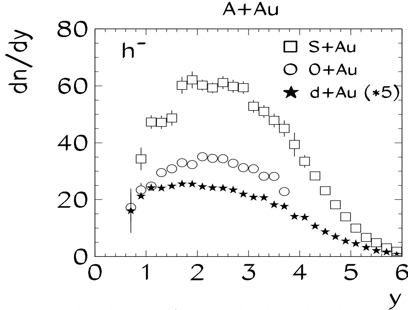
Figure 22. Rapidity distributions of negatively charged hadrons produced in central d+Au, O+Au and S+Au collisions.
