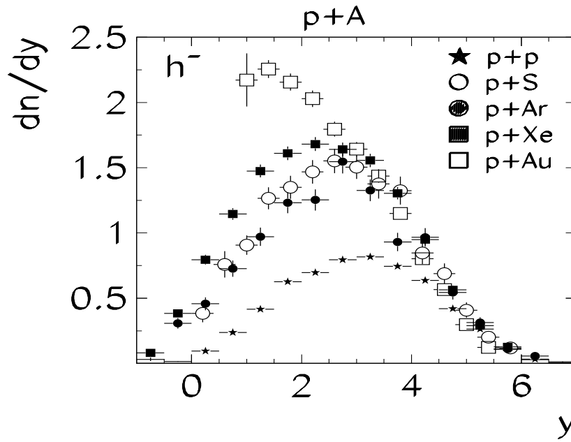
Figure 21. Rapidity distributions of negatively charged hadrons produced in minimum bias p+p , p+S , p+Ar , p+Xe and p+Au collisions [ 36]. Note that the rapidity distribution for p+S collisions is higher than for p+Ar interactions due to different trigger conditions and event selections.
