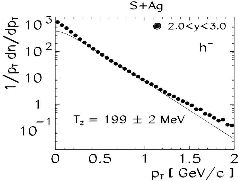
Figure 31. Transverse momentum distribution of negatively charged hadrons produced in central S+Ag collisions. The solid line is a fit of Eq. 2 to the data in the interval 0.3 < p_T < 1.0 GeV/c. The vertical scale is given in (GeV) -2 .
