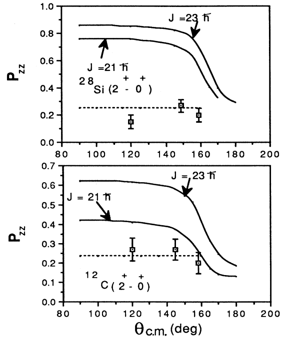
FIG. 11. The spin alignment parameter of 1.78 MeV \gamma rays for -10 < Q < 0 MeV and of 4.44 MeV \gamma rays for -22 < Q < -10 MeV at E_{\text{c.m.}} = 43.5 MeV. The solid curves and dashed lines are statistical and dinuclear orbiting model calculations, respectively, as explained in the text.
