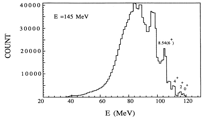
FIG. 3. Singles carbon energy spectrum at \theta_{\text{lab}} = 10^\circ at E_{\text{lab}} = 145 MeV.
