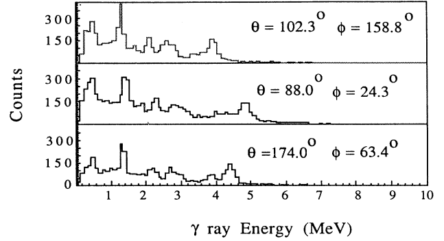
FIG. 9. Coincidence NaI spectra for the reaction ^{28}\text{Si} + ^{12}\text{C} at E_{\text{c.m.}} = 48.0 MeV and -26 < Q < -16 MeV at \theta_{\text{lab}} = 15^\circ , \phi_{\text{lab}} = 0^\circ . Polar and azimuthal angles are measured in a coordinate frame whose Z axis is normal to the reaction plane and X axis is along the beam direction.
