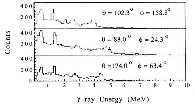
FIG. 10. Coincidence NaI spectra for the reaction ^{28}\text{Si} + ^{12}\text{C} at E_{\text{c.m.}} = 48.0 MeV and -44 < Q < -26 MeV at \theta_{\text{lab}} = 15^\circ , \phi_{\text{lab}} = 0^\circ . Polar and azimuthal angles are measured in a coordinate frame whose Z axis is normal to the reaction plane and X axis is along the beam direction.
