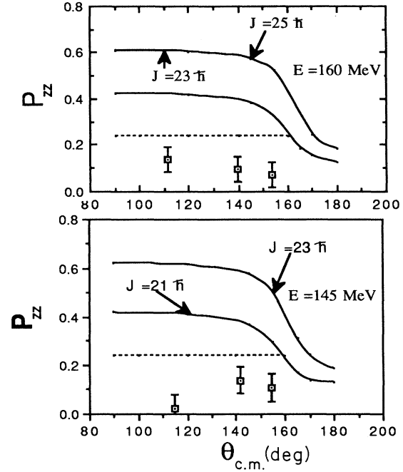
FIG. 13. The spin alignment parameter of 4.44 MeV ^{12}C(2^+ - 0^+) \gamma rays for -40 < Q < -22 MeV at E_{c.m.} = 43.5 MeV and 4.44 MeV ^{12}C(2^+ - 0^+) \gamma rays for -44 < Q < -26 MeV at E_{c.m.} = 48.0 MeV. The solid curves and dashed lines are statistical and dinuclear orbiting model calculations, respectively, as explained in the text.
