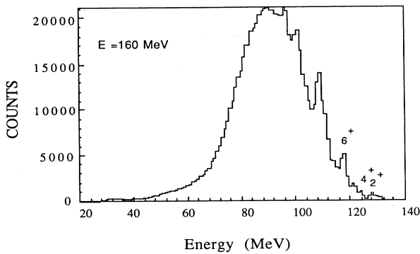
FIG. 7. Singles carbon energy spectrum at \theta_{\text{lab}} = 10^\circ at E_{\text{lab}} = 160 MeV.
