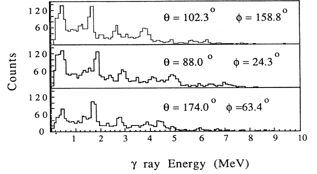
FIG. 8. Coincidence NaI spectra for the reaction ^{28}\text{Si} + ^{12}\text{C} at E_{\text{c.m.}} = 48.0 MeV and -16 < Q < 0 MeV at \theta_{\text{lab}} = 15^\circ , \phi_{\text{lab}} = 0^\circ . Polar and azimuthal angles are measured in a coordinate frame whose Z axis is normal to the reaction plane and X axis is along the beam direction.
