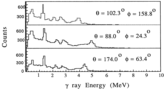
FIG. 6. Coincidence NaI spectra for the reaction ^{28}\text{Si} + ^{12}\text{C} at E_{\text{c.m.}} = 43.5 MeV and -40 < Q < -22 MeV at \theta_{\text{lab}} = 15^\circ , \phi_{\text{lab}} = 0^\circ . Polar and azimuthal angles are measured in a coordinate frame whose Z axis is normal to the reaction plane and X axis is along the beam direction.
