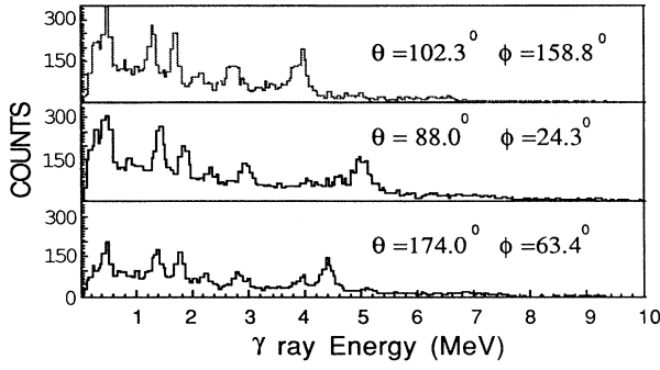
FIG. 5. Coincidence NaI spectra for the reaction ^{28}\text{Si} + ^{12}\text{C} at E_{\text{c.m.}} = 43.5 MeV and -22 < Q < -10 MeV at \theta_{\text{lab}} = 15^\circ , \phi_{\text{lab}} = 0^\circ . Polar and azimuthal angles are measured in a coordinate frame whose Z axis is normal to the reaction plane and X axis is along the beam direction.
