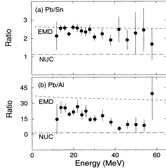
FIG. 14. Ratio of excitation energy spectra. The long-dashed lines represent the expected ratio for pure nuclear behavior. The short-dashed lines represent the ratio obtained with WW photon spectra for pure single photon EMD behavior. (a) Pb/Sn. (b) Pb/Al.
