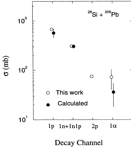
FIG. 6. Measured EMD cross sections (open circles) compared with the calculated cross sections (solid circles) in the WW framework.
