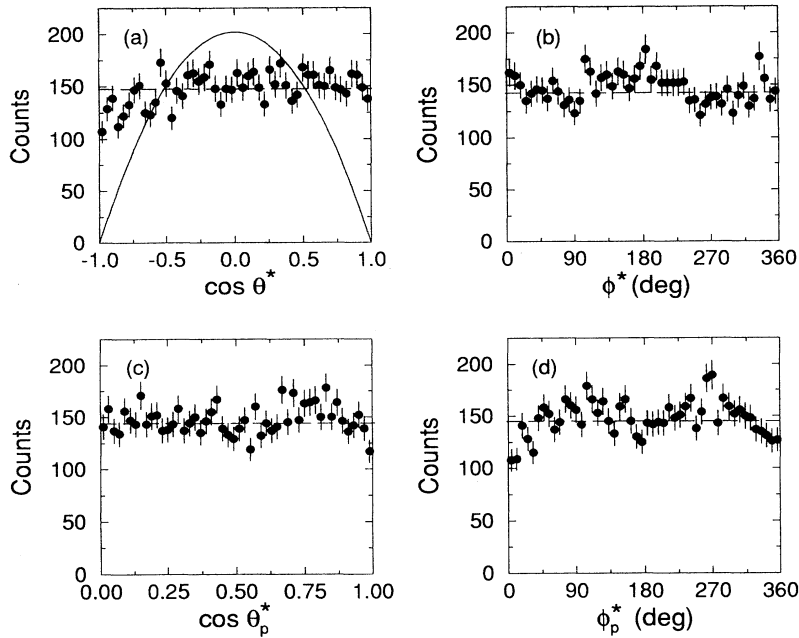
FIG. 12. Angular distributions for the 2p+^{26}\text{Mg} channel. (a) Polar angle of the ^{26}\text{Mg} momentum vector with respect to the beam momentum vector, in the rest frame of the ^{28}\text{Si} projectile. (b) Azimuthal angle of the decay plane about the beam momentum vector in the first two-body decay system, ^{28}\text{Si} \rightarrow \text{"diproton"} + ^{26}\text{Mg} (see text). (c) Polar angle of the momentum vector of the protons with respect to the momentum vector of the diproton, in the rest frame of the diproton (see text). (d) Azimuthal angle of the proton decay plane about the diproton momentum vector. The solid line represents the predicted dependence for spinless projectiles and fragments [13] and the dashed lines are drawn at the mean values of the distributions.
