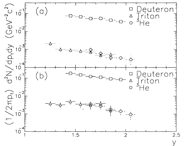
FIG. 4. The invariant yields of deuterons, tritons, and ^3\text{He} at p_t = 0 plotted as a function of rapidity for Si+Pb collisions. Multiplicity cuts correspond to (a) 89% and (b) 8%, respectively, of the geometrical cross section. The uncertainties shown are statistical only.
