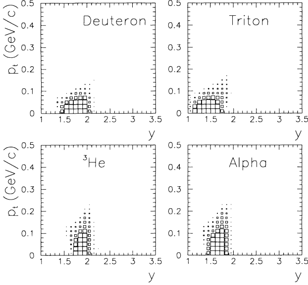
FIG. 2. The acceptance of the E814 apparatus for the detection of deuterons, tritons, ^3\text{He} , and ^4\text{He} . The largest boxes on the plot (sizes vary on a linear scale) correspond to 100% acceptance.
