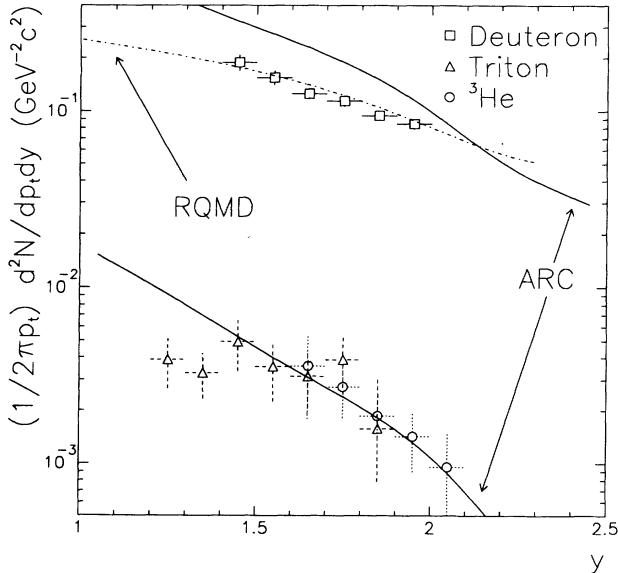
FIG. 9. First results from an ARC coalescence calculation (solid lines) [34] and from an RQMD coalescence calculation (dashed line) [35]. The points are the measured invariant yields at p_t = 0 for 8% \sigma_{\text{geom}} Si+Pb collisions. The ARC curves have been calculated for 7% \sigma_{\text{geom}} in Si+Au collisions for deuterons and mass 3 particles. The RQMD curves are shown for deuterons produced in 8% \sigma_{\text{geom}} Si+Pb collisions.
