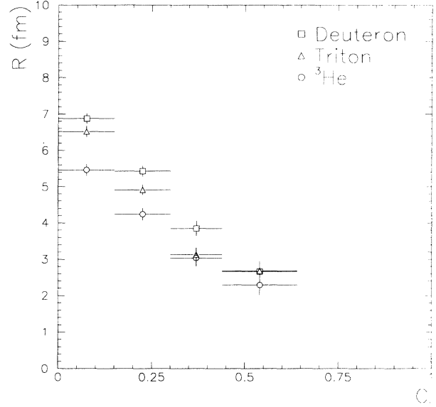
FIG. 8. Radius parameter deduced using the model of Sato and Yazaki [30]. The results are plotted as a function of centrality for deuterons, tritons, and ^3\text{He} created in Si+Pb collisions. The values plotted are averages values of the rms radius for the centrality range represented by the horizontal error bar.
