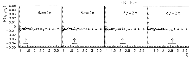
FIG. 10. FRITIOF predictions for correlation function R(\eta_1, \eta_2) for \eta_1 = 1.3 and 2.15 indicated by arrows on the graphs, as a function of \eta_2 . Multiplicity window [120,130] .
