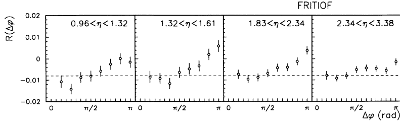
FIG. 15. FRITIOF predictions for the correlation function R(\Delta\phi) as a function of azimuthal angle difference \Delta\phi between two bins of azimuthal angle size \pi/8 for different pseudorapidity regions. Multiplicity window [120,130].
