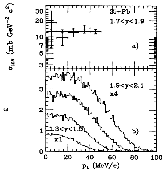
FIG. 2. (a) The invariant cross section \sigma_{\text{inv}} = \frac{1}{2\pi p_t} \frac{d^2\sigma}{dy dp_t} ( \text{mb GeV}^{-2} c^2 ), and (b) the acceptance, \epsilon , of the E814 forward spectrometer plotted as functions of transverse momentum. The four curves are for rapidity bins of width 0.2, starting at y = 1.3 , and have been scaled by factors of 1, 2, 3, and 4.
