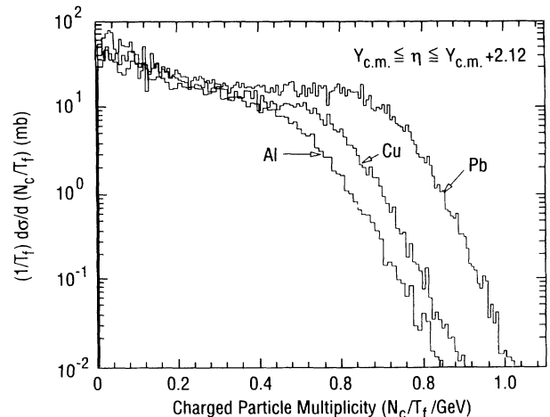
FIG. 17. d\sigma/dN_c for a fixed interval in pseudorapidity relative to Y_{c.m.} for each of the targets. The horizontal axis has been scaled by the maximum center-of-mass kinetic energy available for each of the targets.
