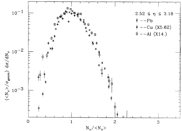
FIG. 16. Relative multiplicity distributions, plotted in KNO variables from the three targets at the same pseudorapidity interval.
