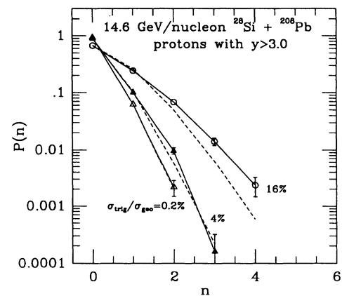
FIG. 6. Probability distribution to find n protons per event for three different levels of centrality obtained by triggering on the TCAL. Data points are connected by solid lines. Also shown as dashed lines are Poisson distributions with the same mean as data.
