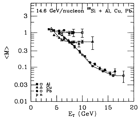
FIG. 5. Average multiplicity of beam rapidity baryons for Si+Al, Cu, and Pb. Solid and open symbols correspond to protons and neutrons, respectively.
