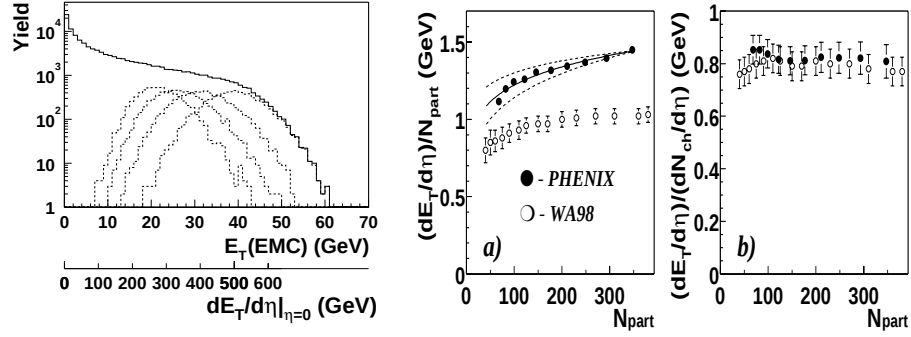
Figure 2. (left) Mid-rapidity dE_T/d\eta|_{\text{mid}} distribution from PHENIX in a solid angle |\eta| < 0.38 , \Delta\phi = 44.4^\circ , corrected to 2\pi in azimuth (solid curve). Dotted curves represent semi-inclusive dE_T/d\eta|_{\text{mid}} distributions for the 4 topmost 5% slices of the of the reference distribution, corresponding to 211, 248, 293 and 347 participants. (right) a) Average mid-rapidity transverse energy per participant in PHENIX ( \sqrt{s_{NN}} = 130 GeV) compared to WA98 ( \sqrt{s_{NN}} = 17.2 GeV); b) Average transverse energy per charged particle versus the number of participants.
