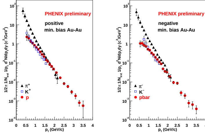
Figure 3. Semi-Inclusive Invariant Yield for Min-Bias Au+Au
