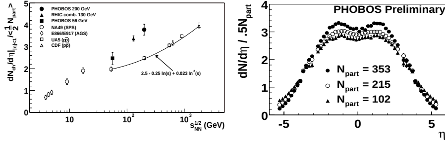
Figure 1. PHOBOS multiplicity. (left) Mid-rapidity dn_{ch}/d\eta|_{mid} per participant pair from RHIC (solid points), lower energy RHI collisions (open points) and p - \bar{p} collisions (open points with line); (right) pseudorapidity distribution of multiplicity per participant pair for 3 different centralities labelled by N_{part} , the deduced number of participants.
