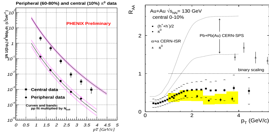
Figure 6. (left) PHENIX semi-inclusive invariant yield of \pi^0 vs p_T for central and peripheral collisions, compared to the pointlike scaling of p-p measurements; (right) R_{AA} , the ratio of the measured charged hadron and \pi^0 p_T spectra to the pointlike scaled p-p data for central collisions compared to lower energy A+A measurements illustrated by data points from \alpha-\alpha at the CERN ISR and by a band representing the CERN-SPS Pb+Pb measurements.
