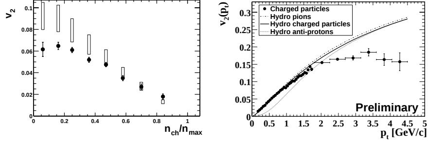
Figure 5. STAR Elliptic flow: (left) v_2 vs centrality (solid points) open boxes are proportional to the eccentricity of the ‘almond’; (right) v_2(p_T) for minimum bias collisions.
