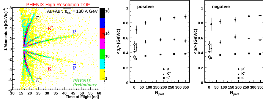
Figure 4. (left) PHENIX Particle I.D. by Time of Flight; (right) Filled points: \langle p_T \rangle vs N_{part} , Open points: \bar{p} - p and p - p data interpolated to \sqrt{s} = 130 GeV.
