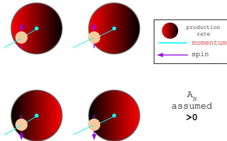
Figure 1.4: Stereoscopic (cross-eyed) illustration of azimuthal asymmetry in forward particle production, or A_N .
