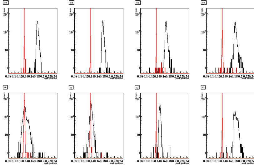
Figure 2.23: 2009 \sqrt{s} = 200 GeV \pi^0 peak position for each sector in the EMCAL before and after the EMCAL tower-by-tower calibration. Sectors E0 and E1 are the PbGL.
