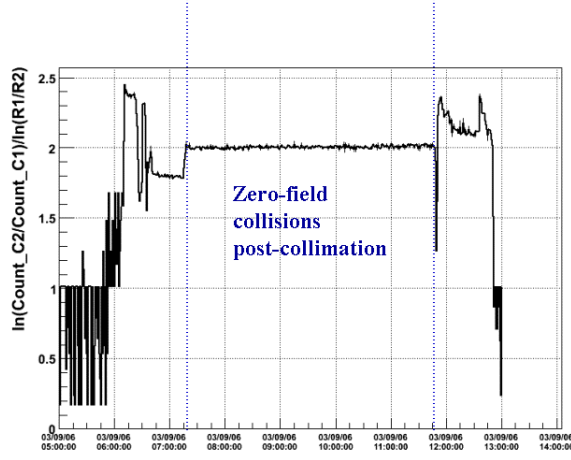
Fig. 21. Ratio R_{rad} = 2 for a zero field run - the post-collimation phase is indicated by the blue vertical lines.
