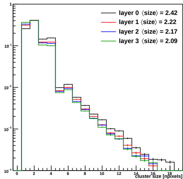
Run 114 -- 120 GeV p -- clusters assoc. w/ 4-hit tracks
