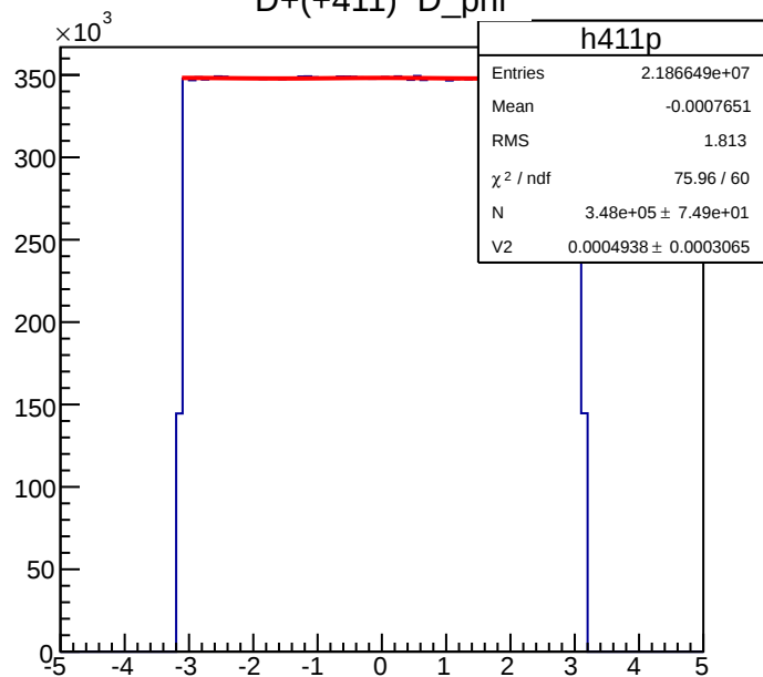
D+(+411) D_phi
