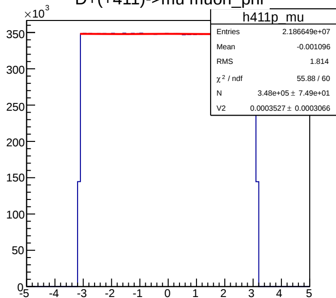
D+(+411)-&gt;mu muon_phi
