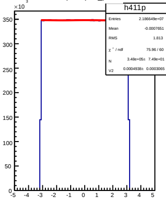
D+(+411) D_phi
