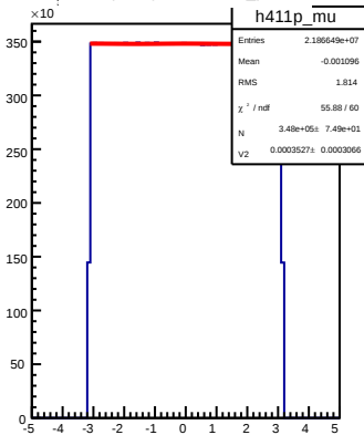
D+(+411)-&gt;muon_phi
