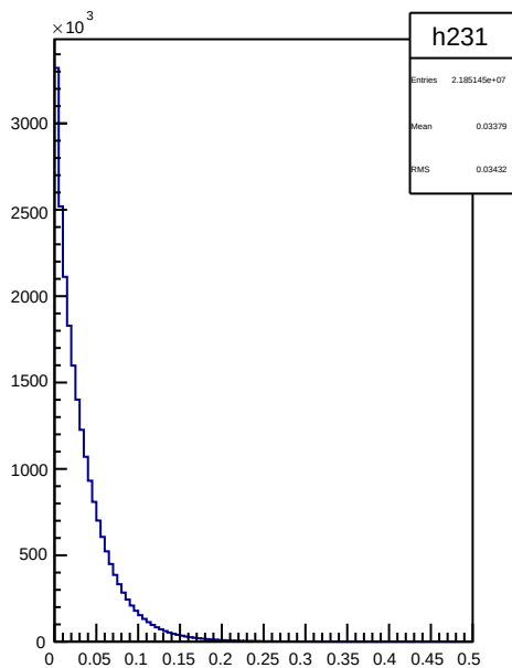
D_xF
