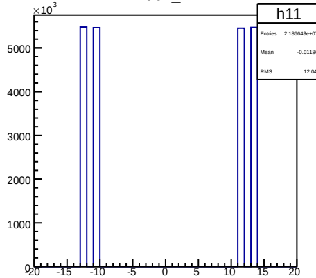
muon_ID
