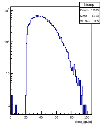
dimu_gpz[0]
