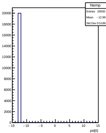
pid[0]
