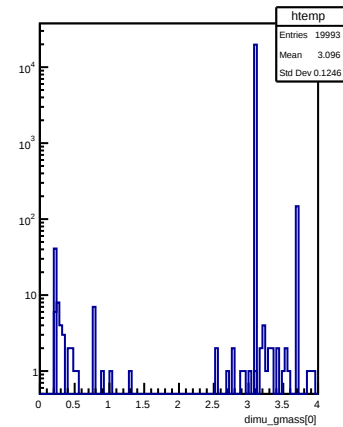
dimu_gmass[0]
