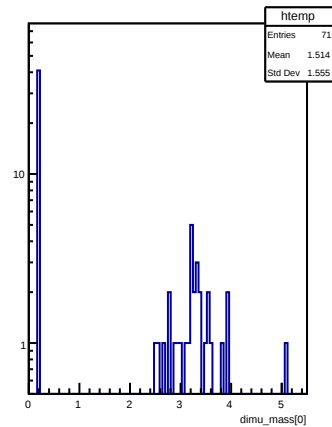
dimu_mass[0] {dimu_mass[0]&lt;100}
