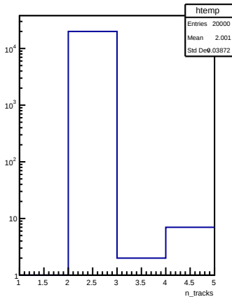
n_tracks
