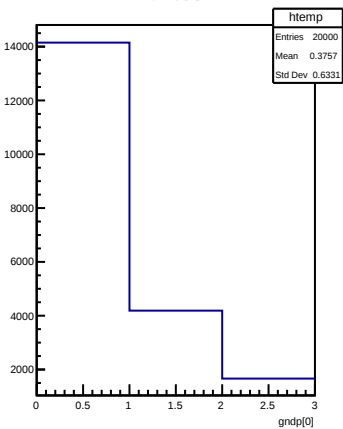
gndp[0]
