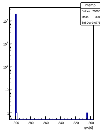
gvz[0]
