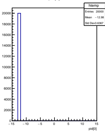
pid[0]
