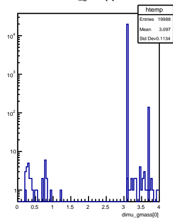
dimu_gmass[0]
