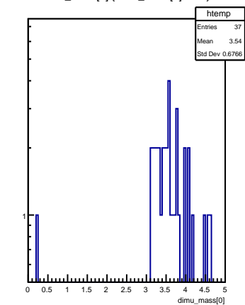
dimu_mass[0] {dimu_mass[0]&lt;100}
