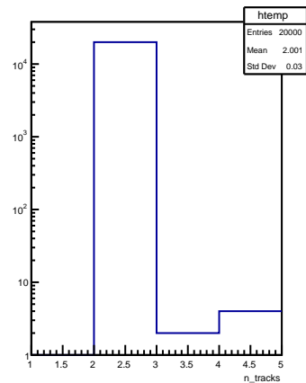
n_tracks
