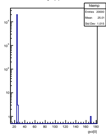
gvz[0]
