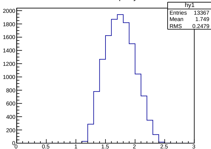
Drell-Yan Rapidity
