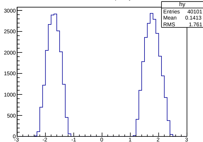
Drell-Yan Rapidity
