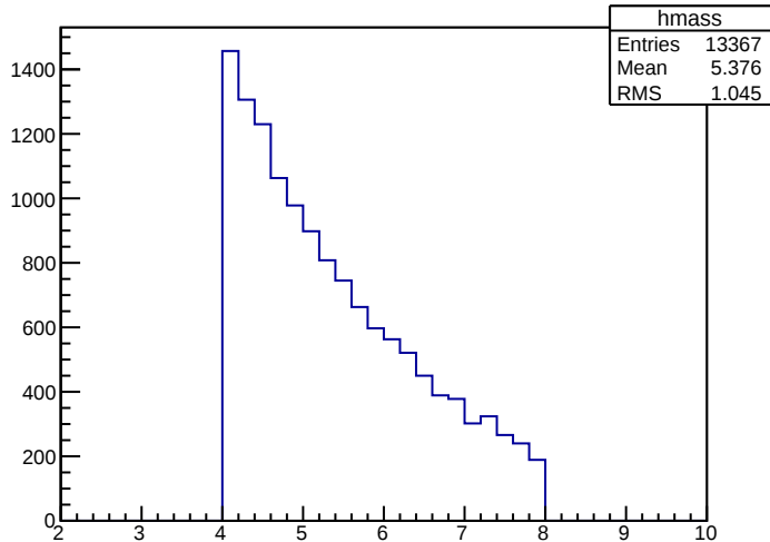
Dimuon Mass
