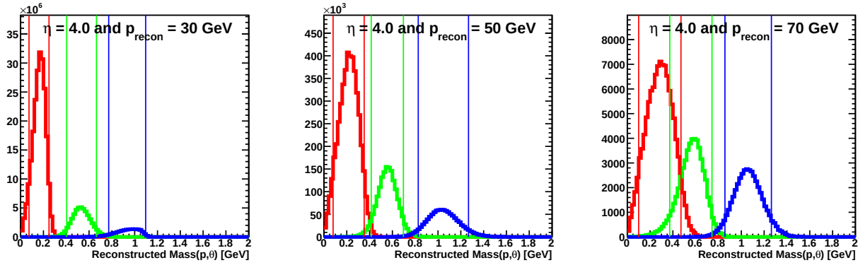
Figure 3.9: Reconstructed mass distribution via m(p, \theta_{Crk}) at \eta = 4 for reconstructed momenta 30 GeV/c (left), 50 GeV/c (middle) and 70 GeV/c (right), for pions (red), kaons (green) and protons (blue), with the parent momentum and particle abundances from the PYTHIA generator. Vertical lines indicate the symmetric mass cuts corresponding to 90% efficiency. Note that particle true momentum is on the average smaller than reconstructed momentum, see Figure 3.10.
