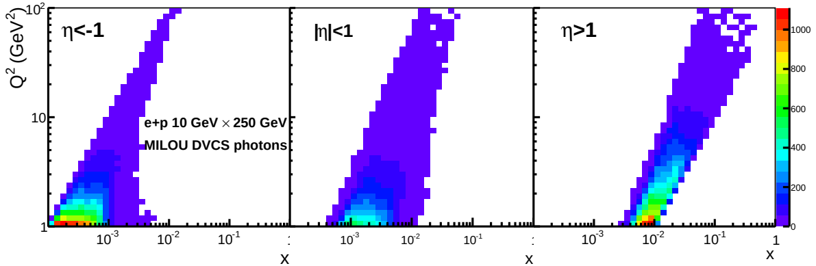
Figure 2.11: For 10 \text{ GeV} \times 250 \text{ GeV} beam energy configuration: x - Q^2 coverage for DVCS events with photon detected in the electron-going direction, \eta < -1 (left), or central rapidities, |\eta| < 1 (middle) and hadron-going direction, \eta > 1 (right). The z-axis scale shows relative distribution of events from the MILOU event generator.
