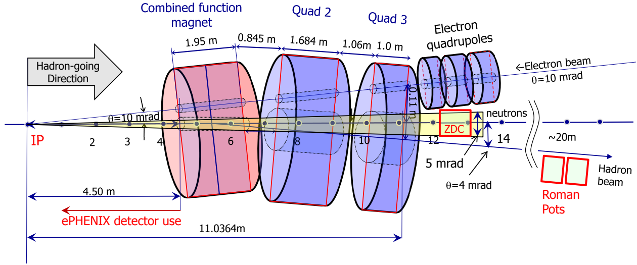
Figure 3.14: Floor plan show the locations for ZDC and Roman Pots relative to the ePHENIX interaction point. One layout of the interaction point magnets are also shown [30].
