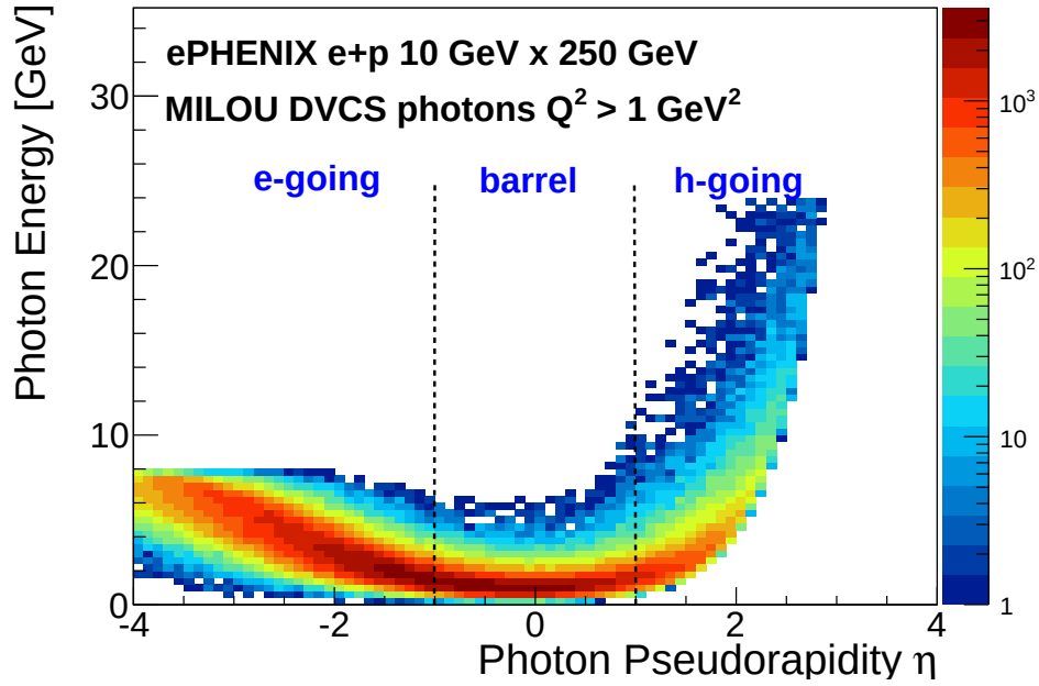
Figure 2.10: For the 10 \text{ GeV} \times 250 \text{ GeV} beam energy configuration: DVCS photon energy vs pseudorapidity distribution; the z-axis scale shows the relative distribution of events from the MILOU event generator.
