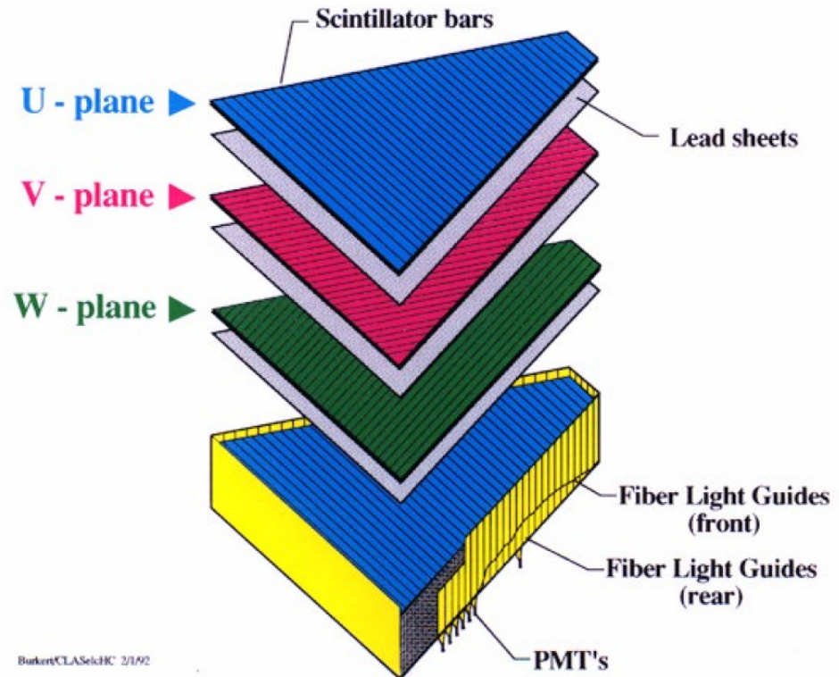
Calorimeter construction:
