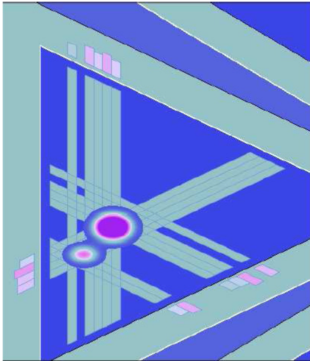
Calorimeter cluster reconstruction (1 sector shown):
