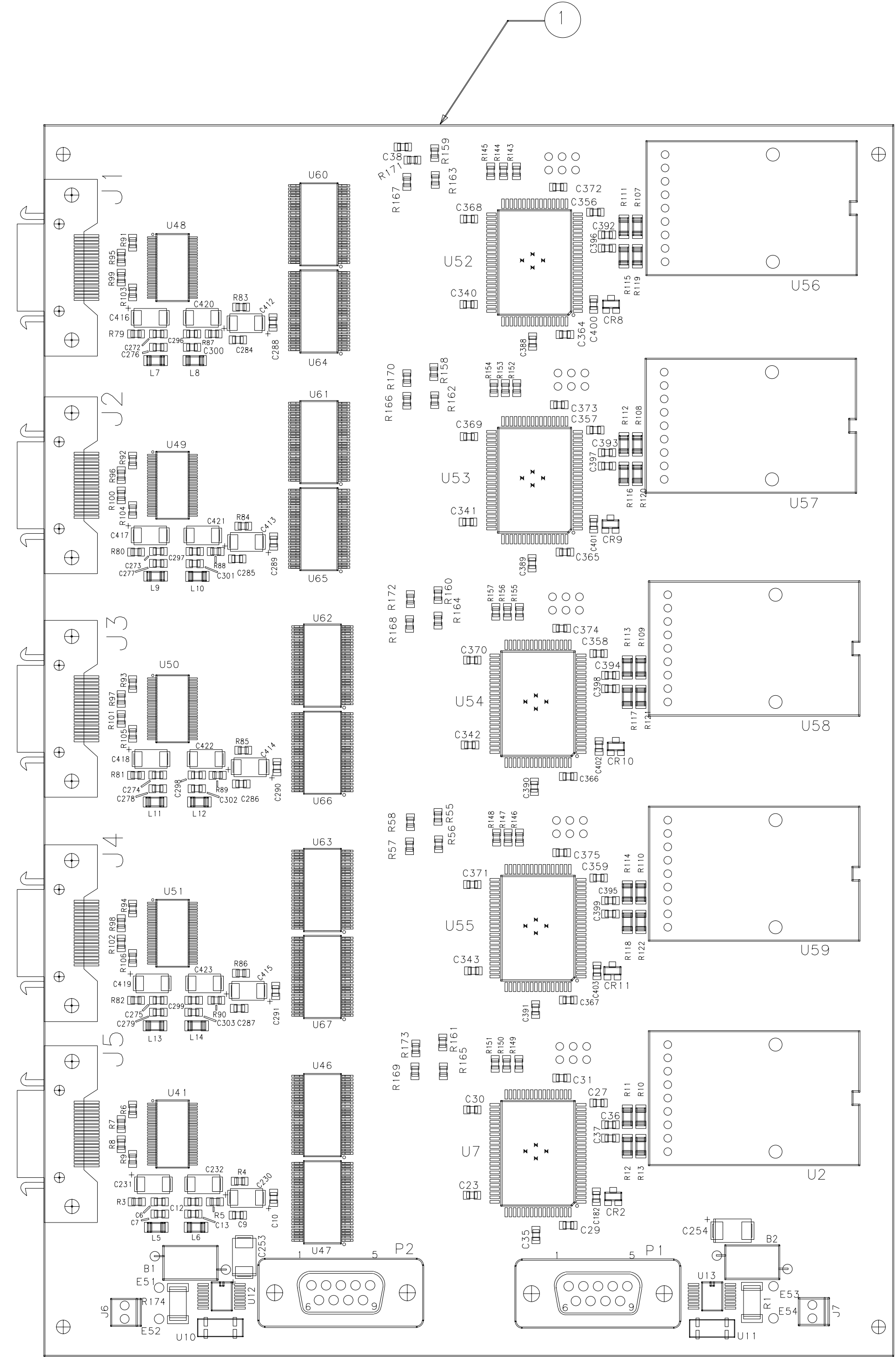
CLINK_RX J01 10Y-226430M09 07-18-00 SILKSCREEN COMPONENT SIDE
