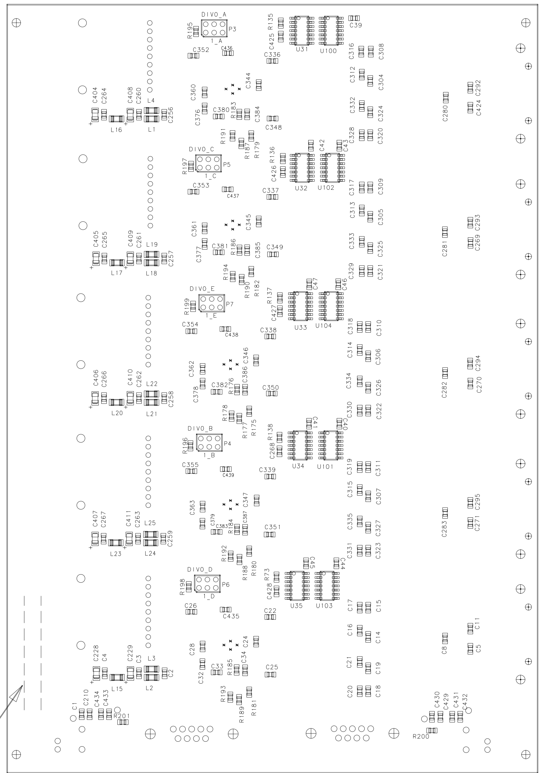
CLINK_RX J01 10Y-226430M10 07-18-00 SILKSCREEN SOLDER SIDE
