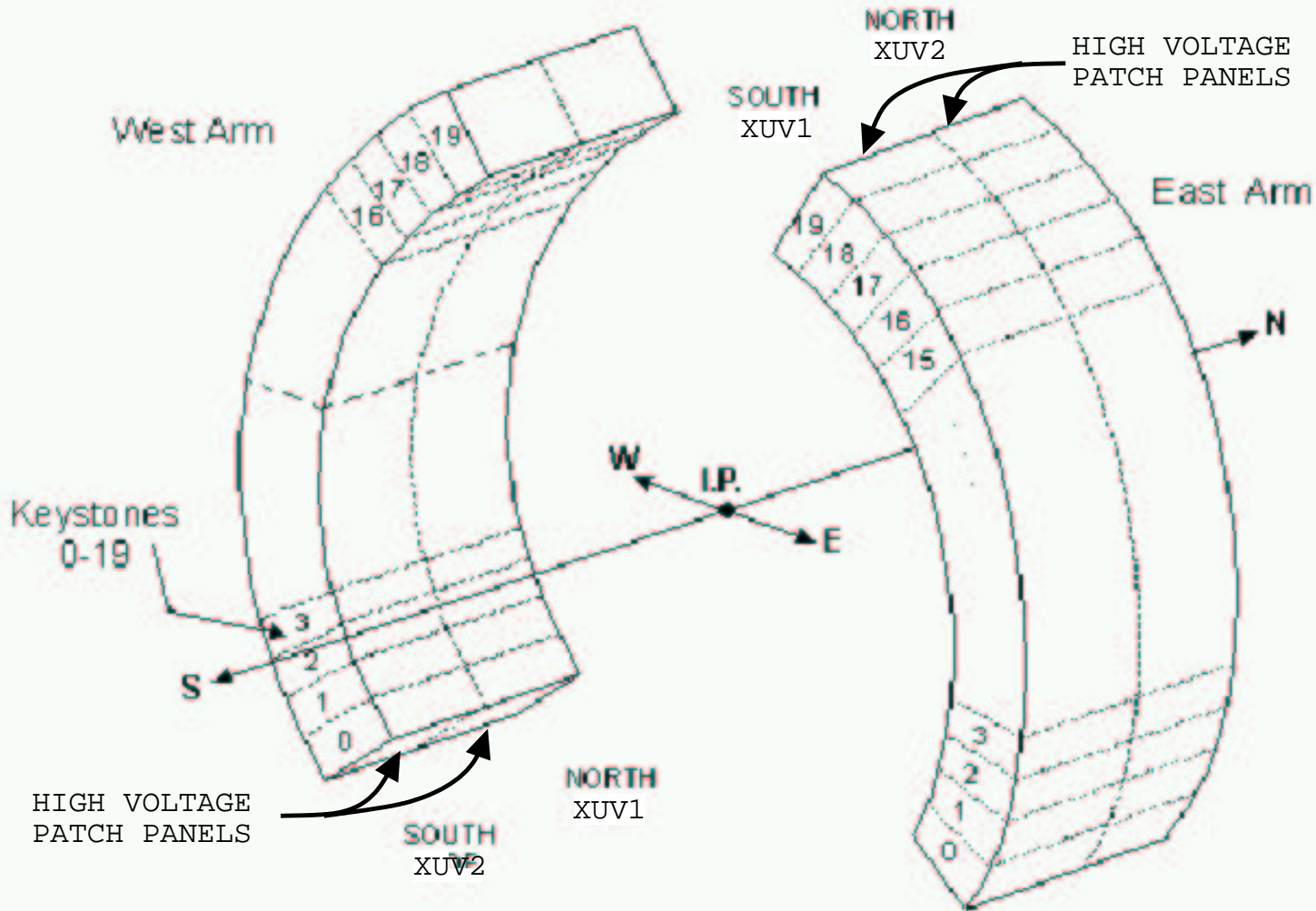
Drift Chamber "keystone" numbering convention
